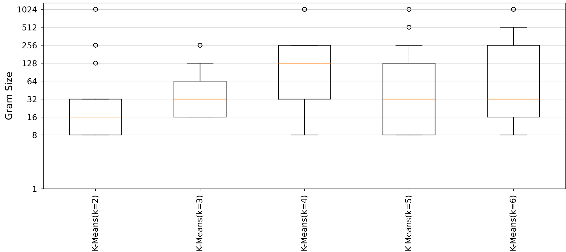
YARA Rules Gram Size Distribution (Cluster32_Size6 dataset)
